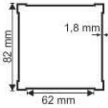
2606 1,625 kg/m
